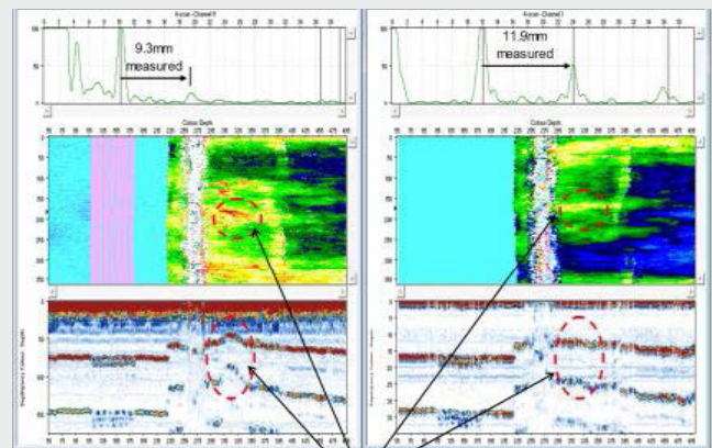
EXAMPLE OF CORROSION MAPPING RESULTS:
