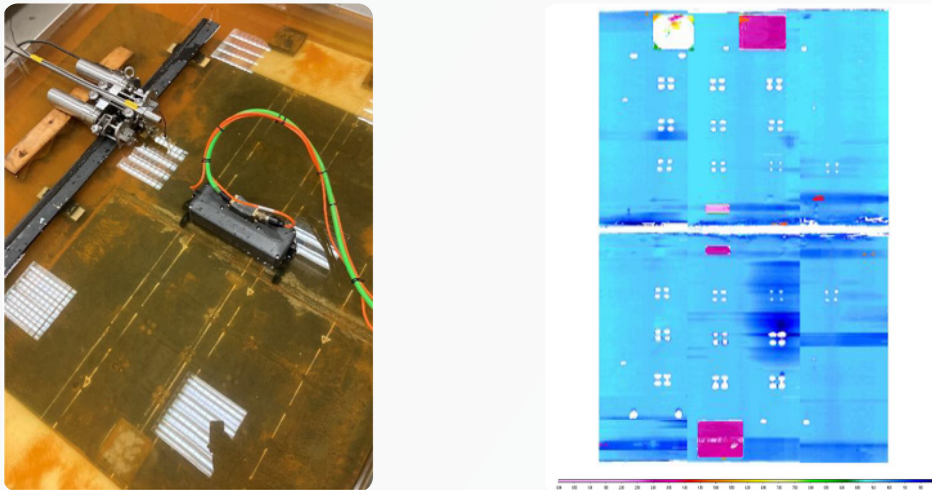
Figure 1: API Qualification Plate and PA MUX System
