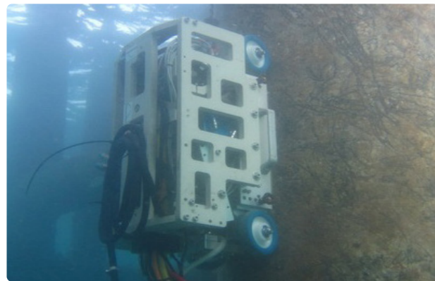
MEC™ - MPS200+ SCANNER
