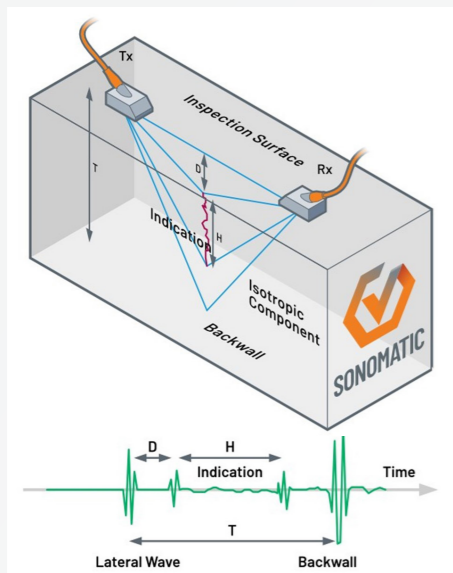
FIGURE 1 - TOFD PRINCIPLE
